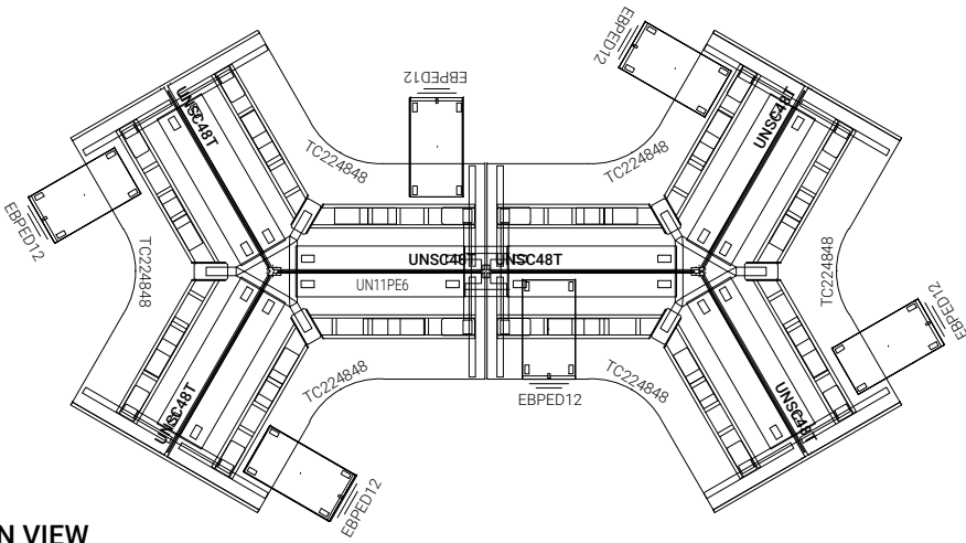
PLAN VIEW Scale: 1/4" = 1'-0"
