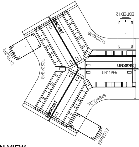
PLAN VIEW Scale: 1/4" = 1'-0"
